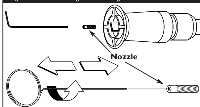
Figure 15 — Removing and Cleaning Nozzle
