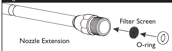
Figure 14 — Clean In-Line Filter
