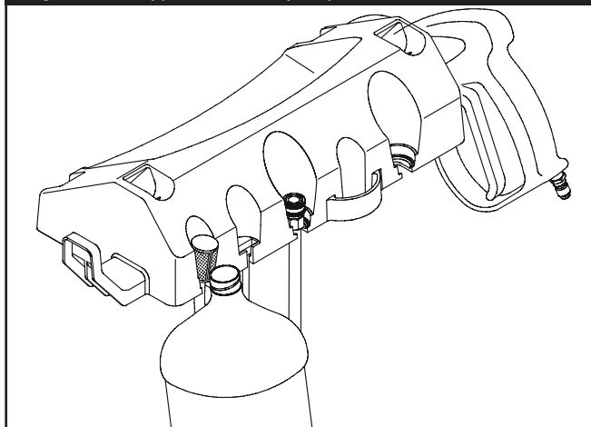
Figure 16 — Typical Accessory Tray
