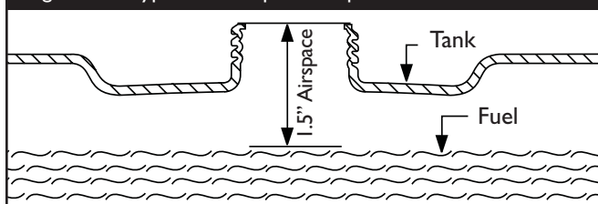
Figure 7 — Typical Fuel Expansion Space
