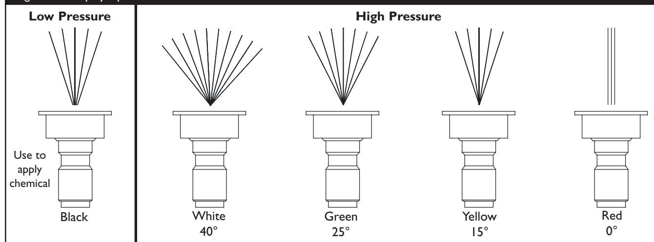
Figure 17 — Spray Tips
