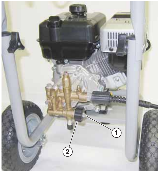
Figure 32 – Water Connection WP3000Z Shown
