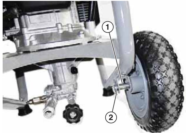
Figure 10 – Installing Wheel Axle
