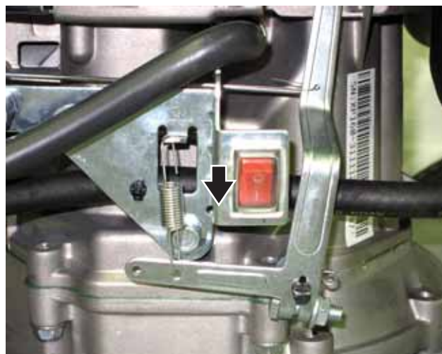
Figure 36 – Engine Stop Switch ON Position
