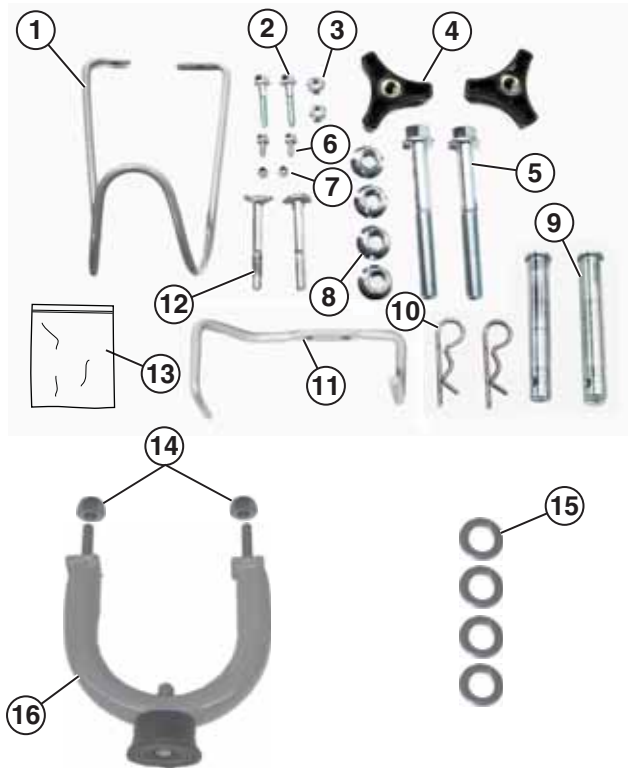
Figure 5 – Hardware
