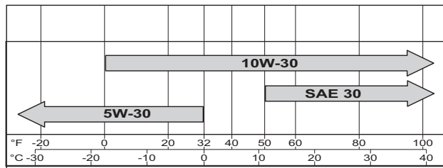
Figure 48 – Recommended Oil
