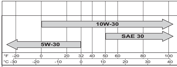
Figure 52 – Recommended Oil
