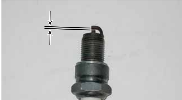
Figure 67 – Spark Plug Gap Requirements
