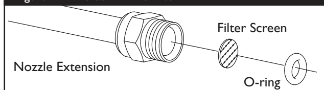
Figure 19 — Clean In-Line Filter
