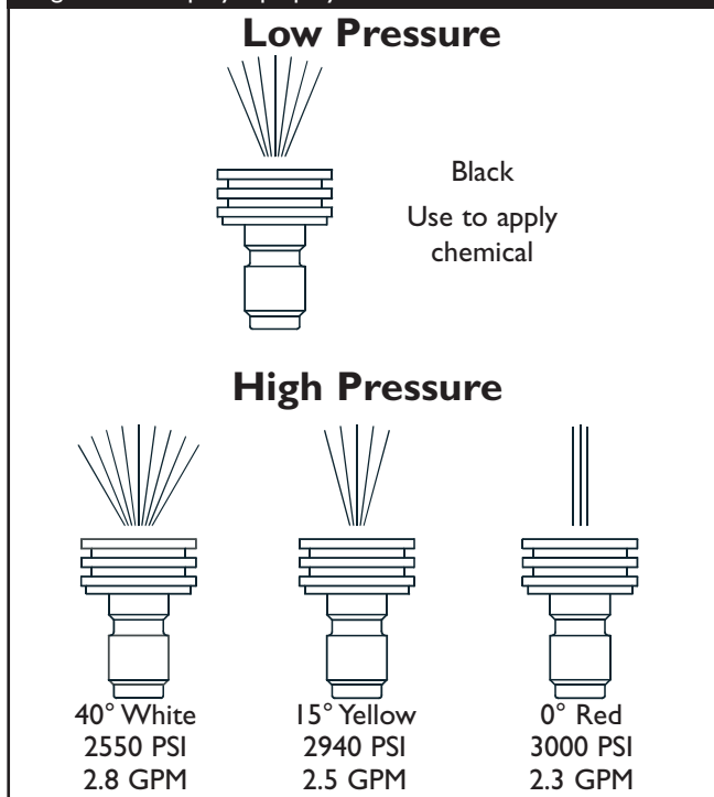
Figure 13 — Spray Tip Spray Patterns
