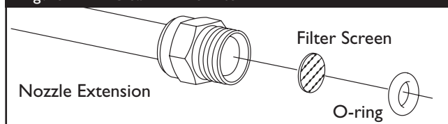
Figure 21 — Clean In-Line Filter
