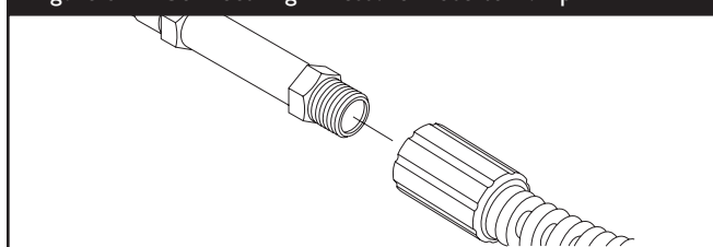
Figure 5 — Connect High Pressure Hose to Pump
