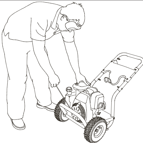
Figure 11 - Recommended Starting Position
