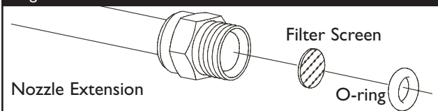
Figure 14 — Clean In-Line Filter
