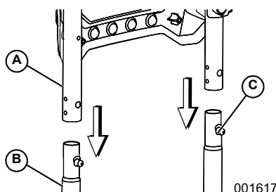
Figure 2-1. Insert Handle
