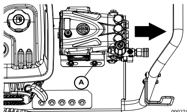
Figure 3-13. Pull Pump Away From Engine
