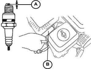
Figure 3-19. Spark Plug
