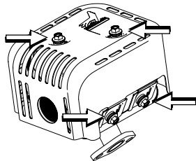
Figure 3-20. Heat Shield Fasteners
