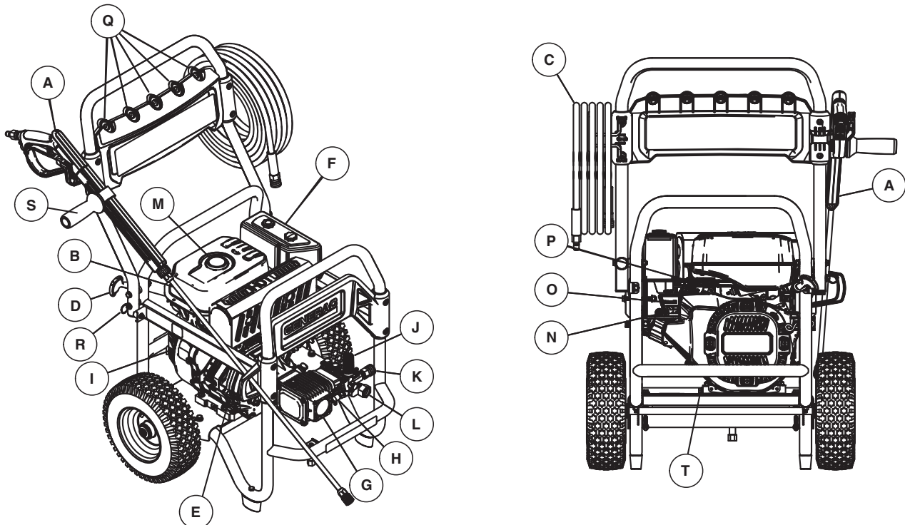
Figure 1 – Features & Controls
