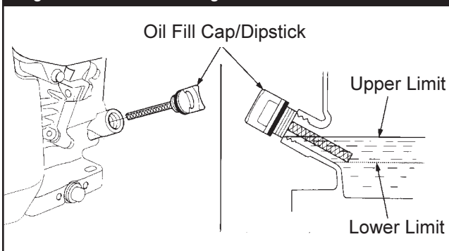
Figure 2 — Add Oil to Engine Crankcase
