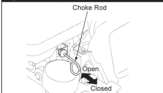
Figure 8 — Choke positions
