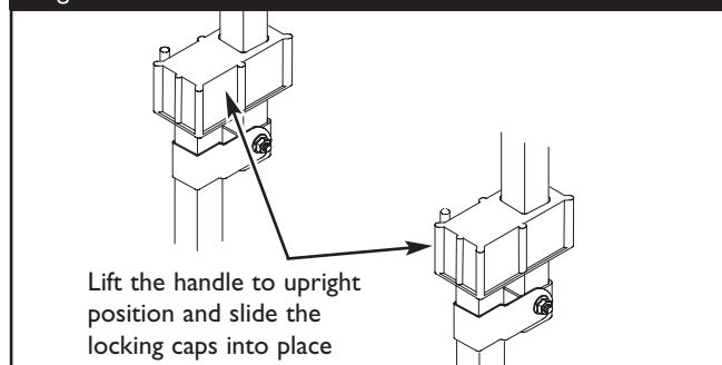
Figure 4 - Secure Handle
