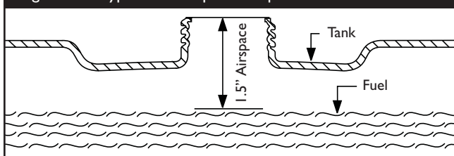
Figure 6 — Typical Fuel Expansion Space
