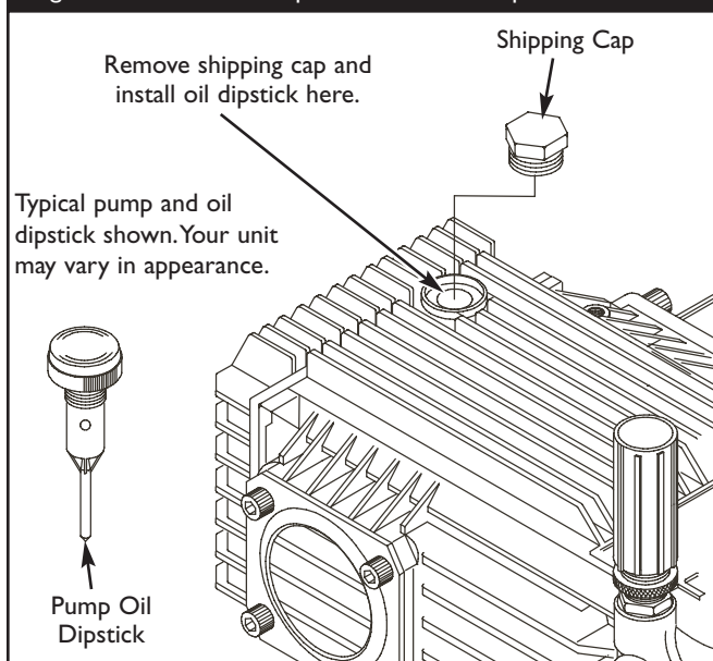
Figure 5 — Install Oil Dipstick onto the Pump
