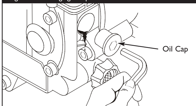
Figure 19 - Changing Pump Oil
