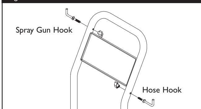
Figure 3 — Attach "L" Hooks to Handle
