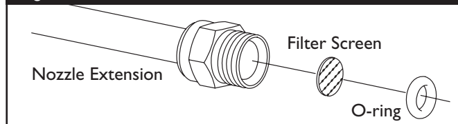
Figure 10 — Clean In-Line Filter
