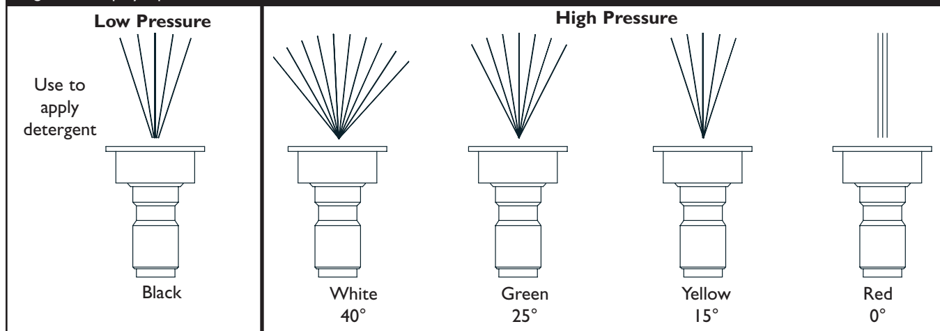
Figure 9 — Spray Tips
