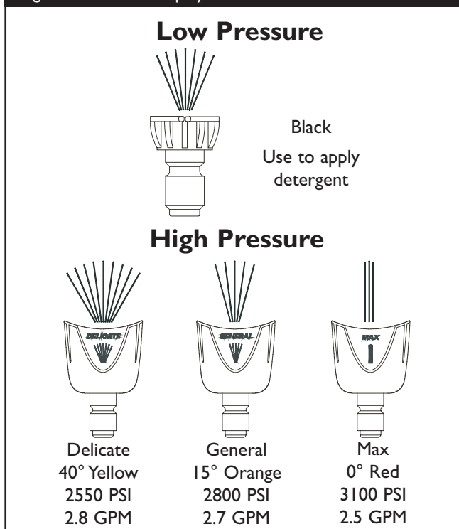
Figure 15 — Nozzle Spray Patterns
