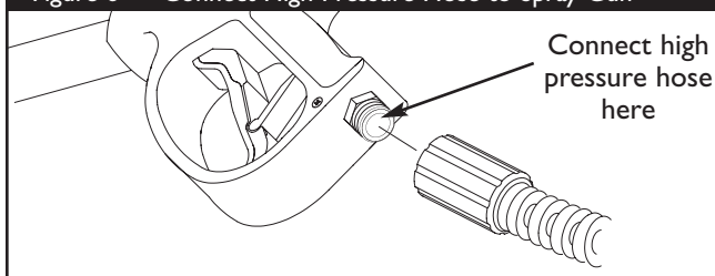
Figure 6 — Connect High Pressure Hose to Spray Gun
