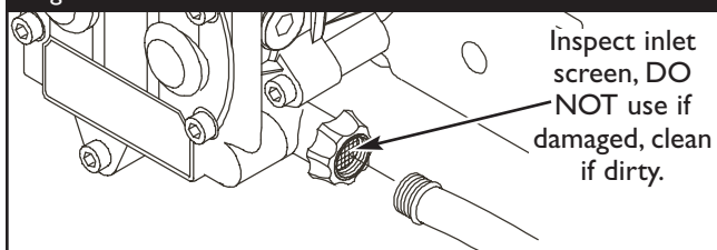
Figure 8 — Connect Garden Hose to Water Inlet
