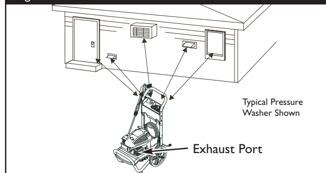
Figure 9 — Pressure Washer Clearance
