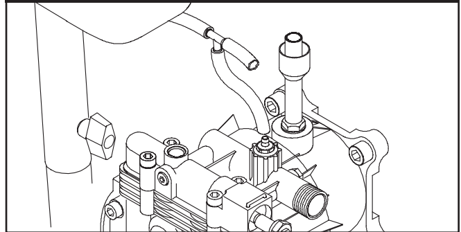
Figure 5 — Attach Chemical Hose to Chemical Injection Fitting on Pump
