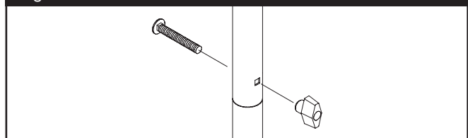
Figure 2 — Secure Handle
