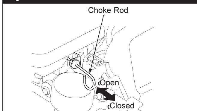
Figure 8 — Choke Positions
