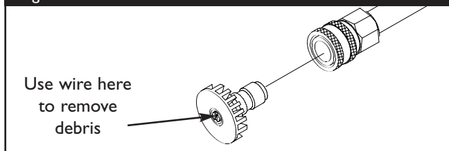
Figure 10 — Nozzle Maintenance
