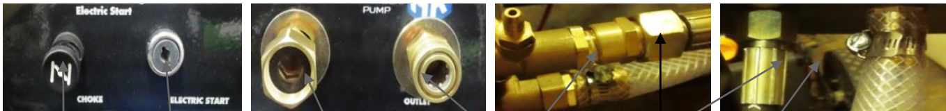
Choke Key Switch Electric Start On/Off Switch for Recoil Start Models Inlet from panel to pump Outlet from panel to pump
