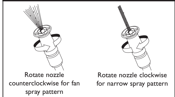
Figure 12 — Adjusting the Nozzle for Spray Pattern
